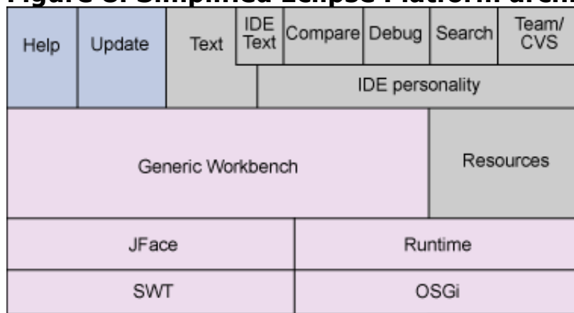
Figure 8. Simplified Eclipse Platform architecture
